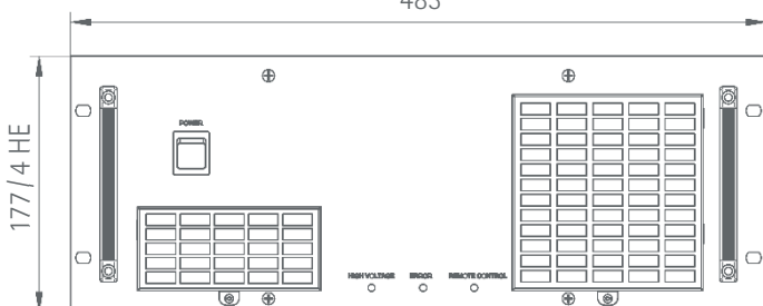
Front view 483
